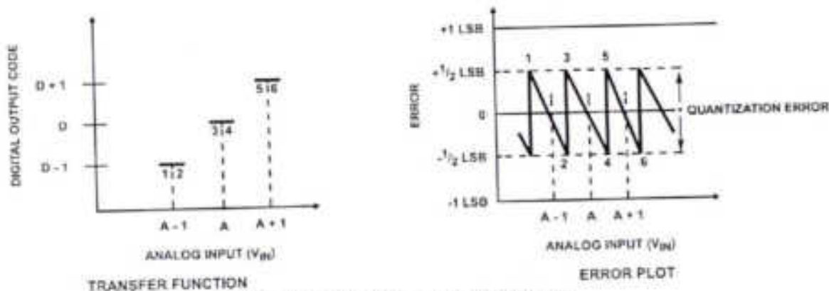
FIGURE 11A. ACCURACY = \pm 0.5 LSB; PERFECT A/D
