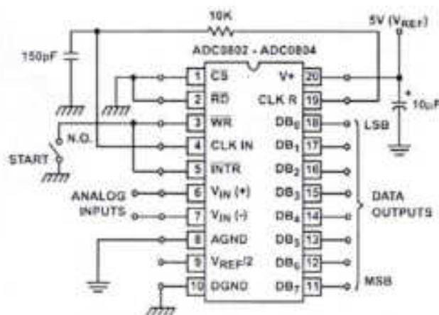
FIGURE 17. FREE-RUNNING CONNECTION
