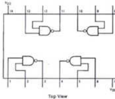
Pin Assignments for DIP and SOIC CD4011BC
