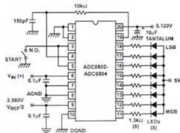
FIGURE 18. BASIC TESTER FOR THE A/D
