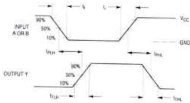
Figure 1. Switching Waveforms
