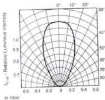
Fig. 3 - Relative Luminous Intensity vs. Angular Displacement
