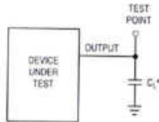
Figure 2. Test Circuit
